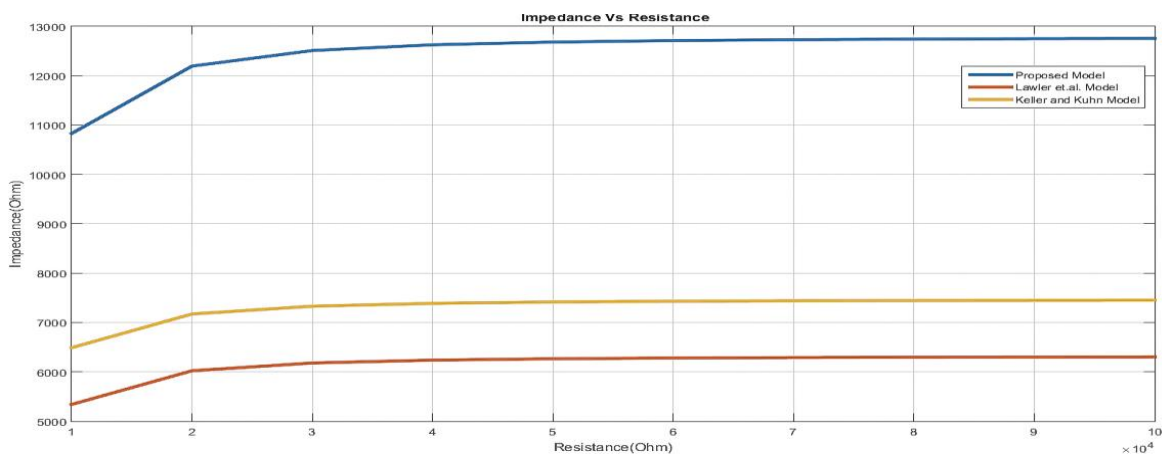
Figure 6. Impedance Vs Resistance of proposed model, Lawler et al and Keller and Kuhn from 10-100 K
