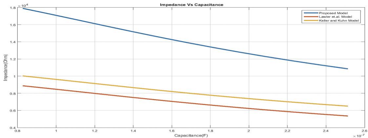
Figure 7. Impedance Vs Capacitance of proposed model, Lawler et al and Keller and Kuhn from 83-251 nF
