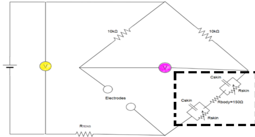
Figure 4. The proposed equivalent circuit for simulation is blocked with the black dashed line
