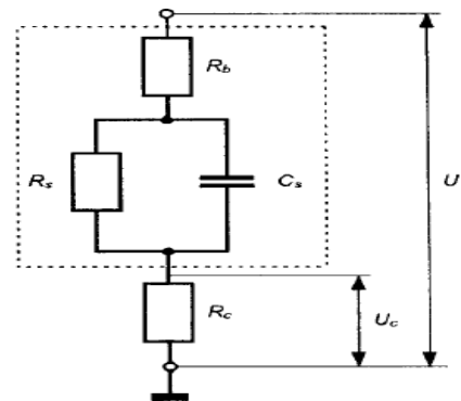
Figure 3. Simple lumped skin model
