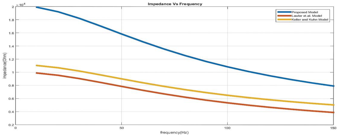
Figure 5. Impedance Vs Frequency of proposed model, Lawler et al and Keller and Kuhn from 10-150 Hz
