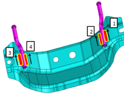
Figure 5. A side of measurement of welding dimension from each point.
