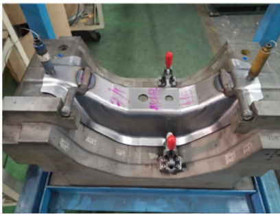
Figure 4. The measurement preparation of welding dimension by jig checking fixture.
