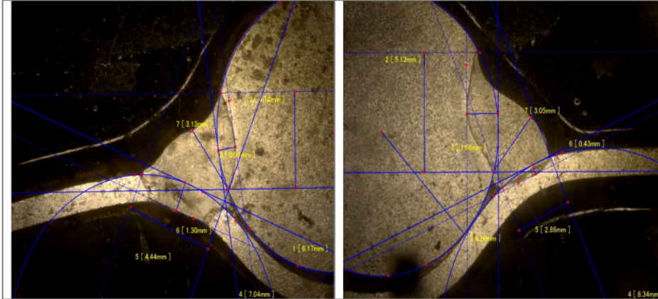
Figure 1. Judgment standard of the ideal welding shape [10].
