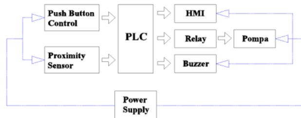
Gambar 7. Diagram blok prototipe
