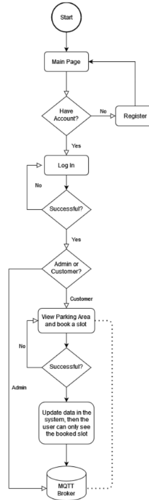
Fig. 2. Flowchart for the reservation scenario
