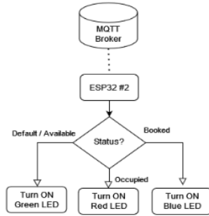
Fig. 4. Flowchart for the indicator of the slot
