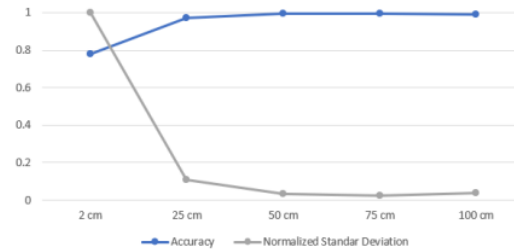
Fig. 5. Statistical summary of ultrasonic sensors test
