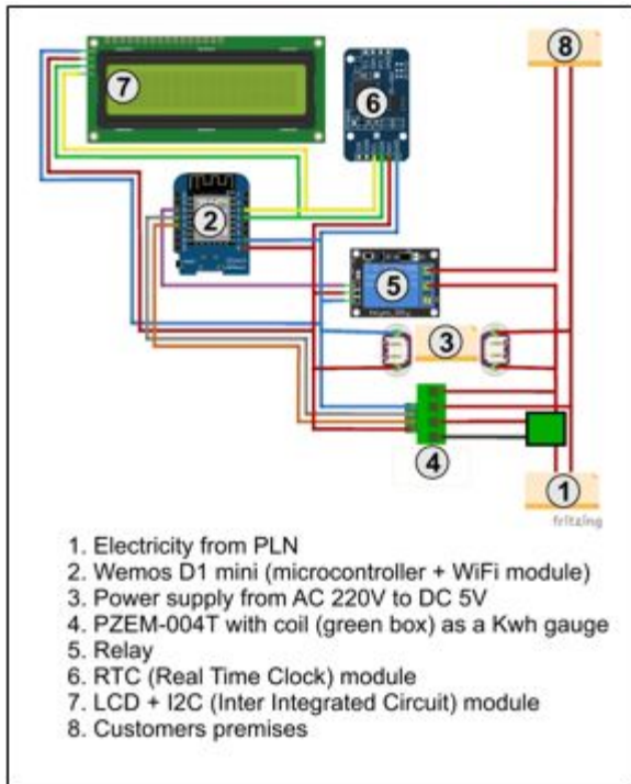
Fig. 1. Main circuit design
