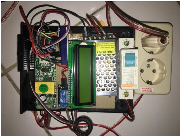
Fig. 2. System hardware
